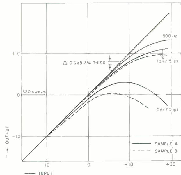
Figure 4. Saturation characteristics at high and low frequencies for different speeds and different modern high-output low noise oxides.
