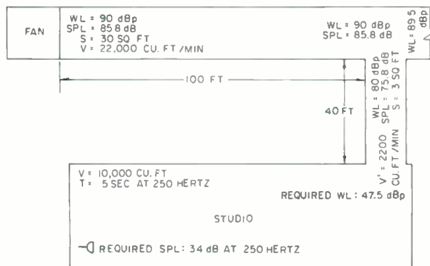
Figure 3. Duct-silencer.
